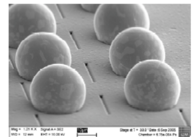
SnAg microbump (20 \mu\text{m} diameter)
